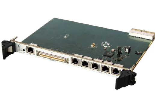
Figure 3. SDM device.
