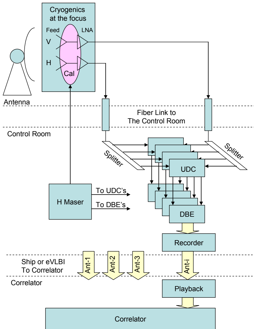
Figure 4-1. VLBI2010 block diagram.
