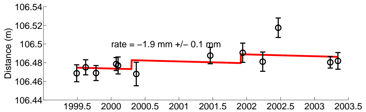
Figure 2. Time series of the distance between the VLBI and GPS monuments at Yebes. From García-Espada et al. (2008)
