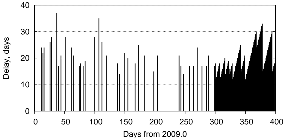
Figure 1: Delay of IVS combined EOP.
