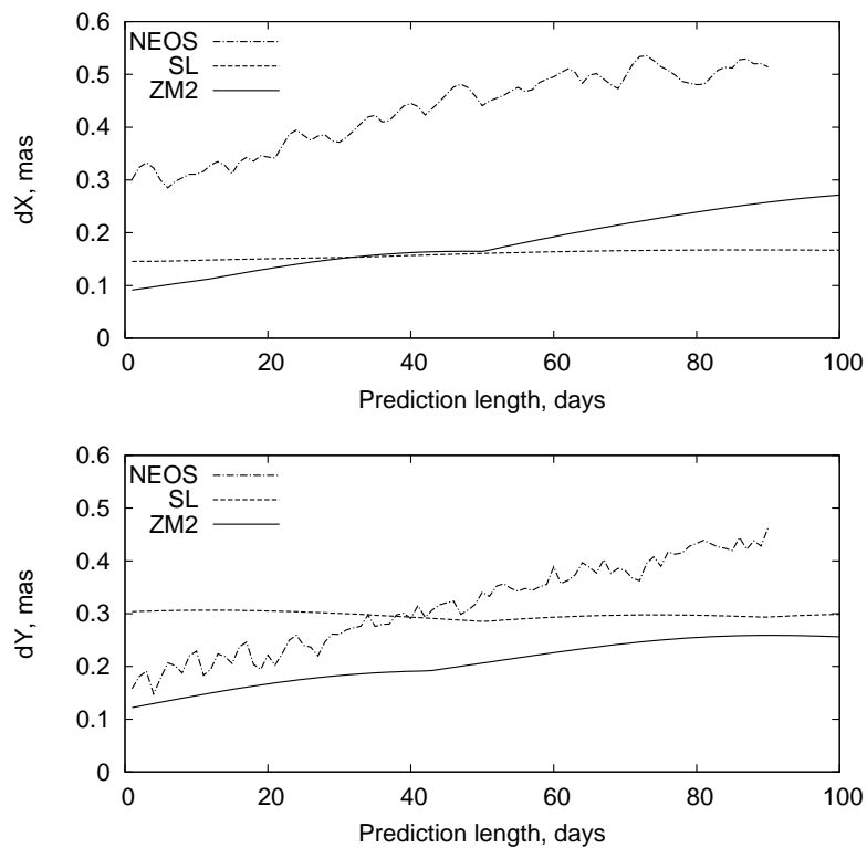
Figure 4: The maximum absolute error of CPO prediction for different models.
