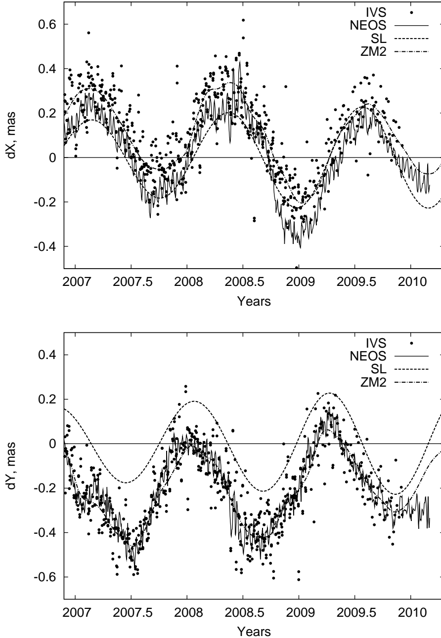
Figure 2: CPO models compared with the IVS combined CPO series.
