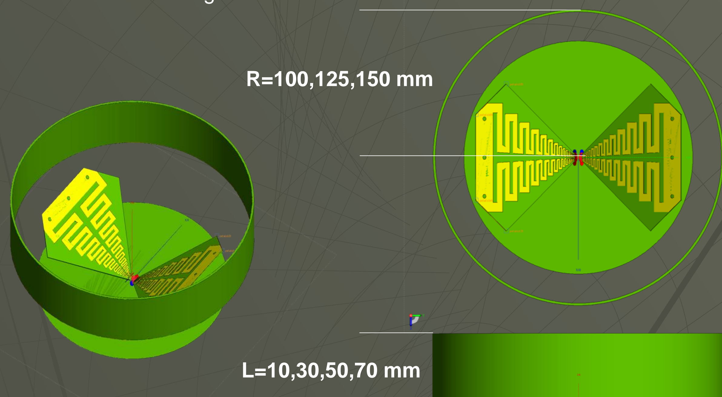
Figure 3: Geometric Model Used to Study Feed Efficiency Dependence on the Cryostat Size
