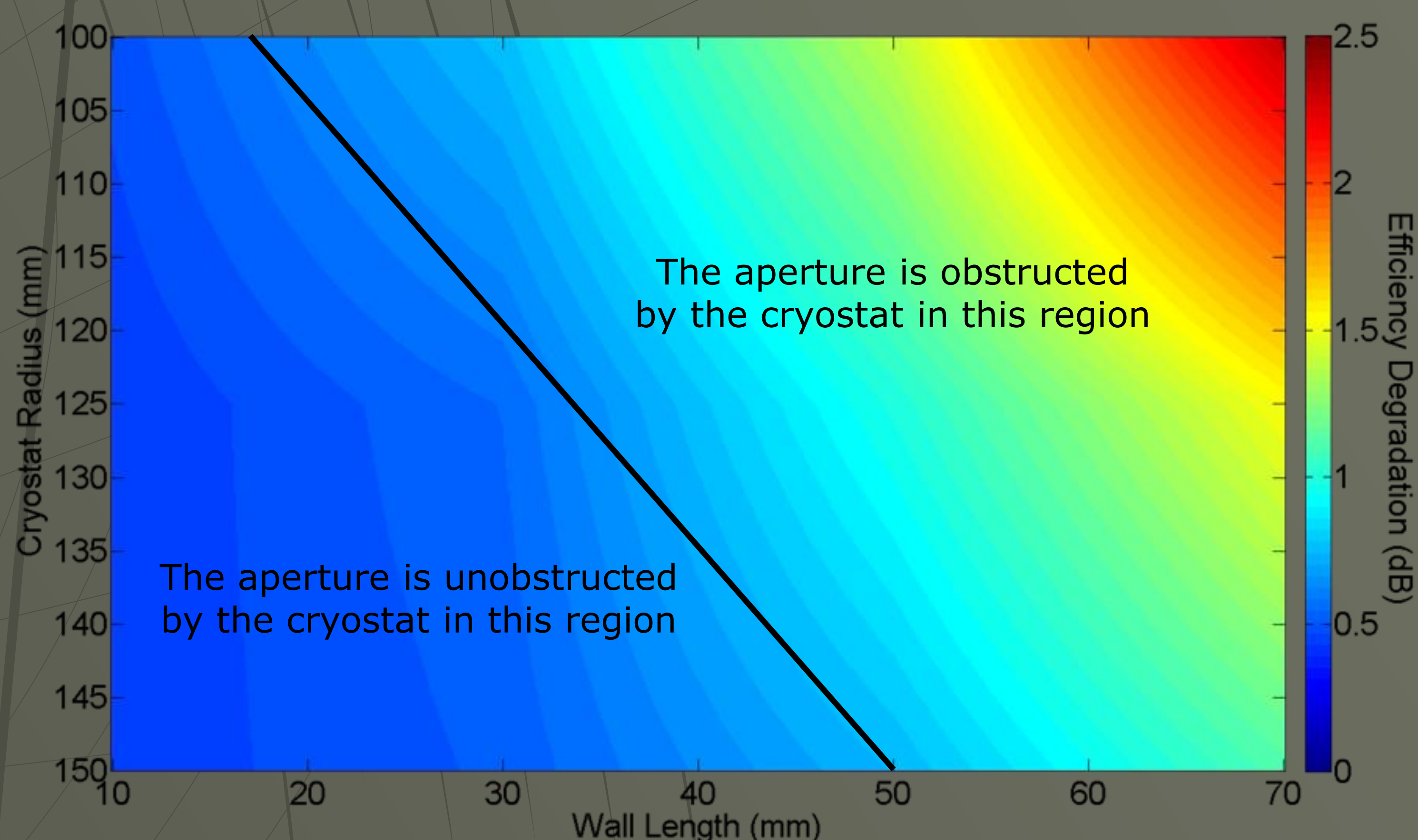
Figure 4: Feed Efficiency Dependence on the Cryostat Size
