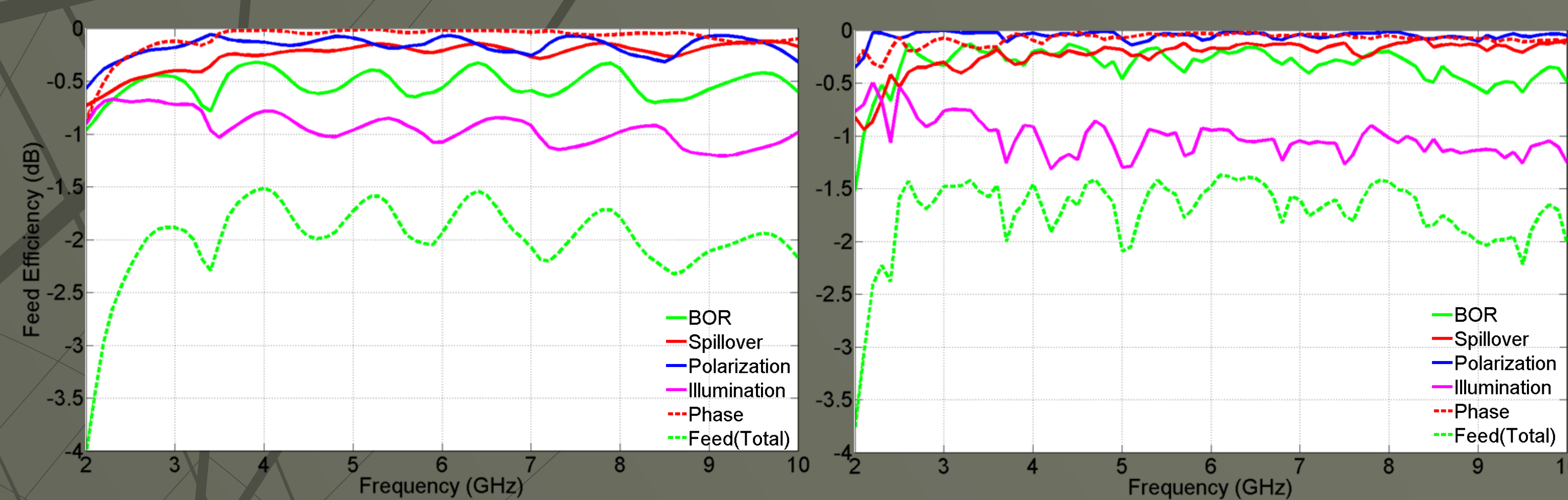
Figure 2a: Eleven Antenna Feed Efficiencies Based on FEKO Model Figure 2b: Eleven Antenna Feed Efficiencies Based on Measurements
