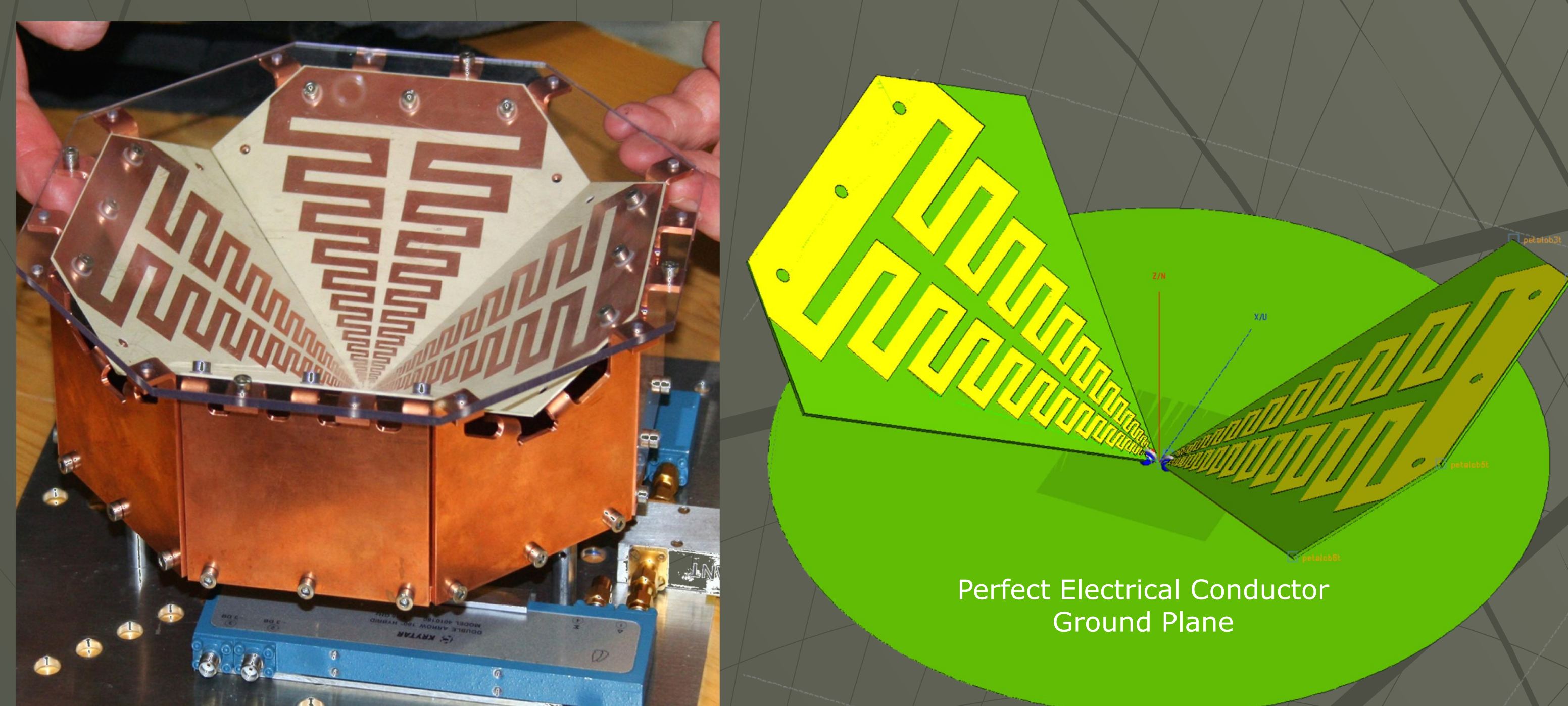
Figure 1a: 2-14 GHz Cryogenic Eleven Feed Figure 1b: Geometric Representation of the Eleven antenna used for Computations
