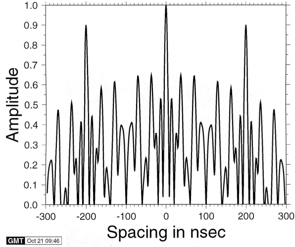
Figure 4: Central part of delay resolution function with 8 channels at X band.
