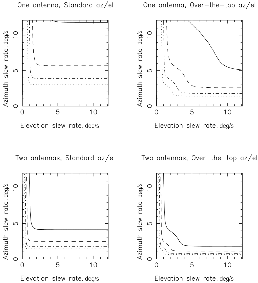
Figure 2. Azimuth vs elevation slew rate to achieve 3D rms position errors (as predicted by the OCCAM Monte Carlo simulator using an optimized uniform sky schedule). The solid line is for 1 mm position error; the dashed line 1.25 mm; the dashed-dotted line 1.50 mm; and the dotted line 1.75 mm. In all cases, 3 \text{ deg/s}^2 slew acceleration is assumed for both axes. All slew rate combinations above and to the right of a line achieve the level of performance of that line
