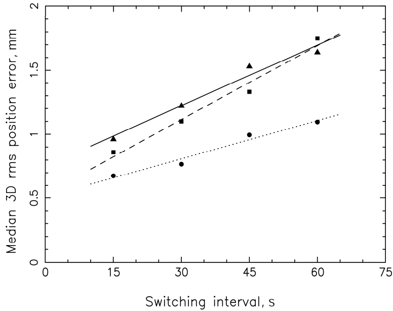
Figure 1. Median 3D rms position error vs Switching interval. The solid line and triangles are for the Solve Monte Carlo simulation; the dashed line and squares are for the OCCAM simulation; and the dotted line and circles are for the PPP simulation
