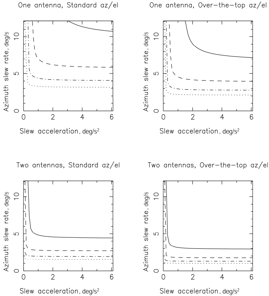
Figure 3. Azimuth slew rate vs acceleration to achieve 3D rms position errors (as predicted by the OCCAM Monte Carlo simulator using an optimized uniform sky schedule). The solid line is for 1 mm position error; the dashed line 1.25 mm; the dashed-dotted line 1.50 mm; and the dotted line 1.75 mm. Elevation slew rates are set to 0.33 of the azimuth slew rate for the standard mount and equal to the azimuth slew rate for the over-the-top mount. All azimuth slew rate and acceleration combinations above and to the right of a line achieve the level of performance of the line
