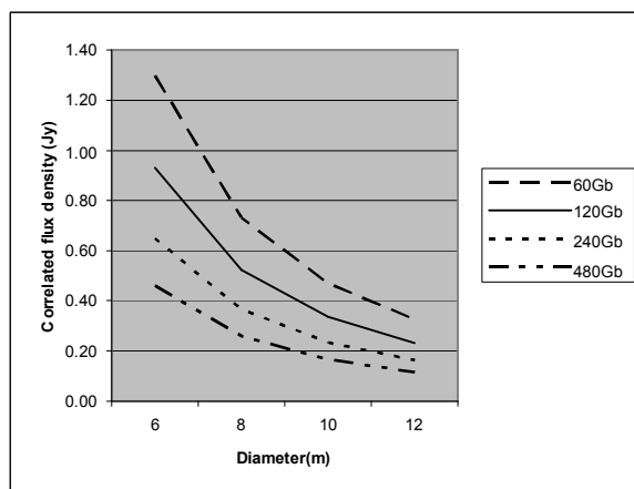
Figure 1: Antenna diameter required to reach an SNR of 24 as a function of correlated flux density for various per-antenna scan-data volumes (for example, 120 Gb is equivalent to a scan of 1 Gbps for 120 sec, 2 Gbps for 60 sec, etc); antennas in the VLBI network are assumed to be identical with T_{\text{sys}}=45\text{K} , efficiency=60%.
