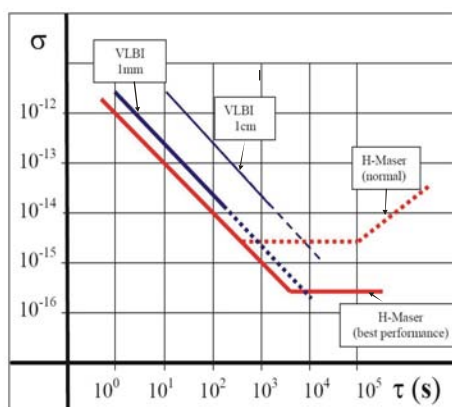
Figure 2: VLBI requirements versus H-maser stability
