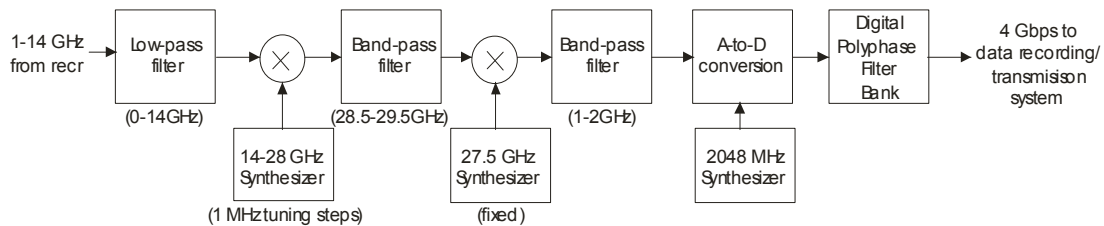
Figure 4: Simplified RF-to-baseband module block diagram
